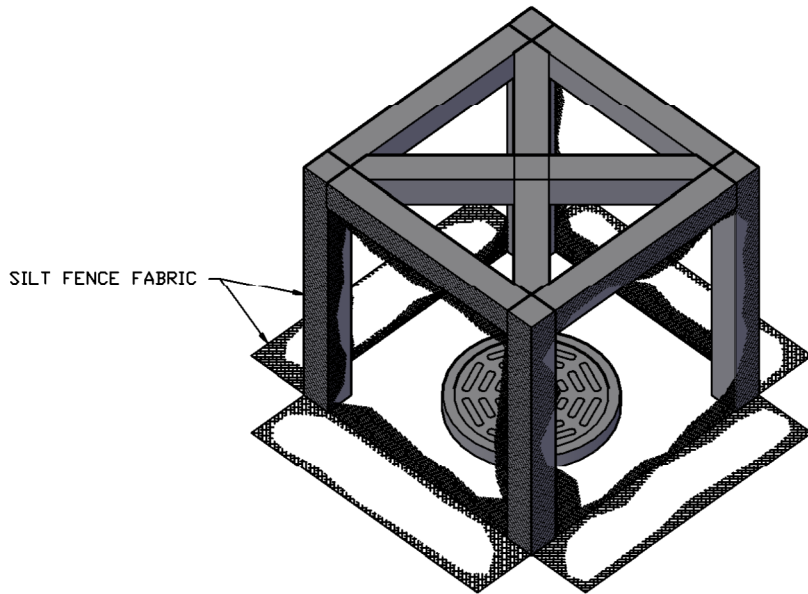
3D VIEW
